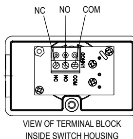
Figure 2: Wiring Diagram
