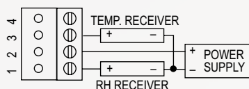
Models with 4-20 mA RH output, with or without 4-20 mA temperature output
