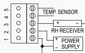
Models with 0-5 V or 0-10 V RH output and a passive thermistor temperature sensor
